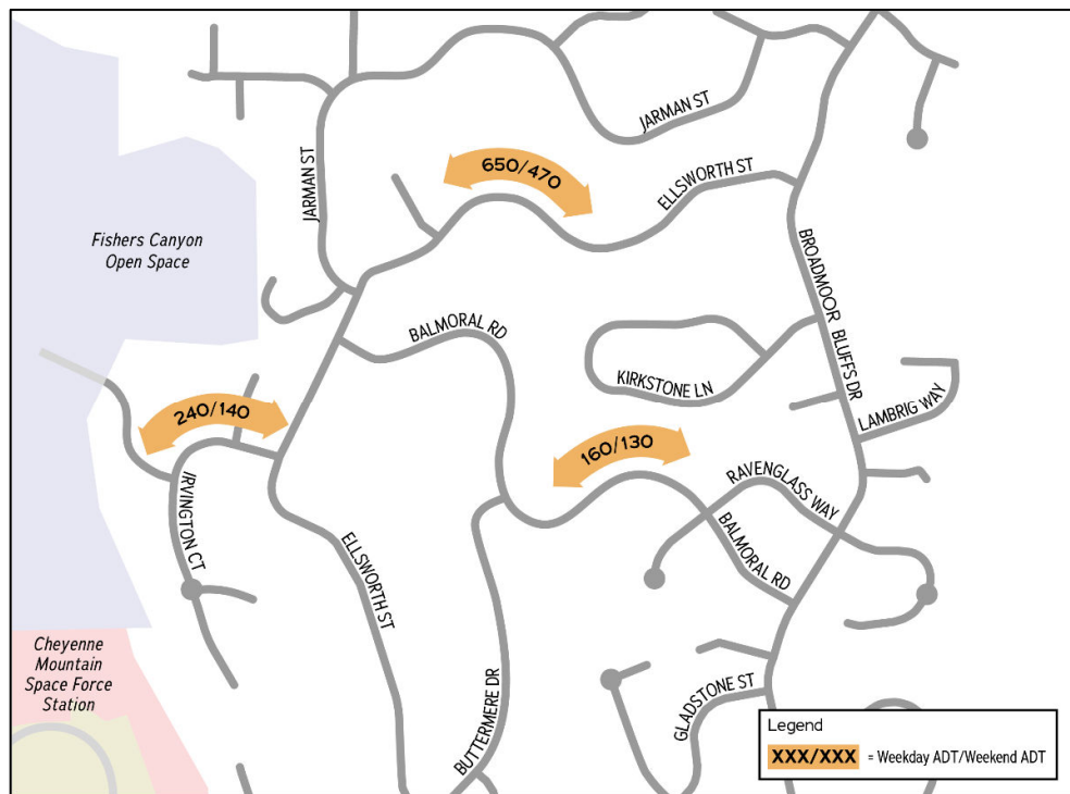
Figure 2-2 - Bidirectional Weekday/Weekend Average Daily Traffic
