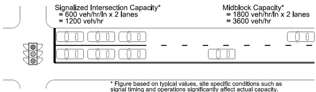
Figure 3: Comparison of Midblock and Signalized Intersection Capacity
